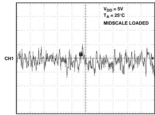
Figure 28. 1/f Noise, 0.1 Hz to 10 Hz Bandwidth
