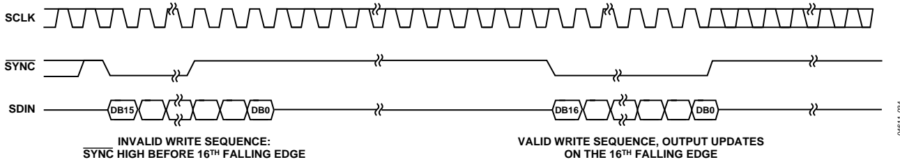
Figure 36. \overline{SYNC} Interrupt Facility
